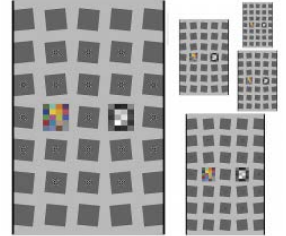
SFRplus Test Charts on Color High-Precision LVT Film
