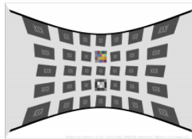
SFRplus Automotive Test Chart
