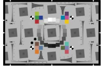
ISO 12233: 2014 Edge SFR (eSFR) chart with extra wedges
