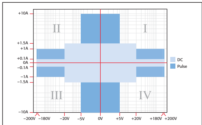
Models 2634B, 2635B, and 2636B I-V capability
