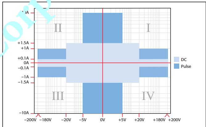
Models 2611B, 2612B, and 2614B I-V capability
